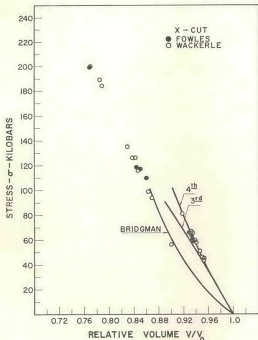
Fig. 7. Stress-volume states resulting from shock compression of X-cut quartz. Solid curve is Bridgman's hydrostatic data. Curves labeled 3rd, 4th are fits based on zero-pressure elastic constants to third- and fourth-order.
