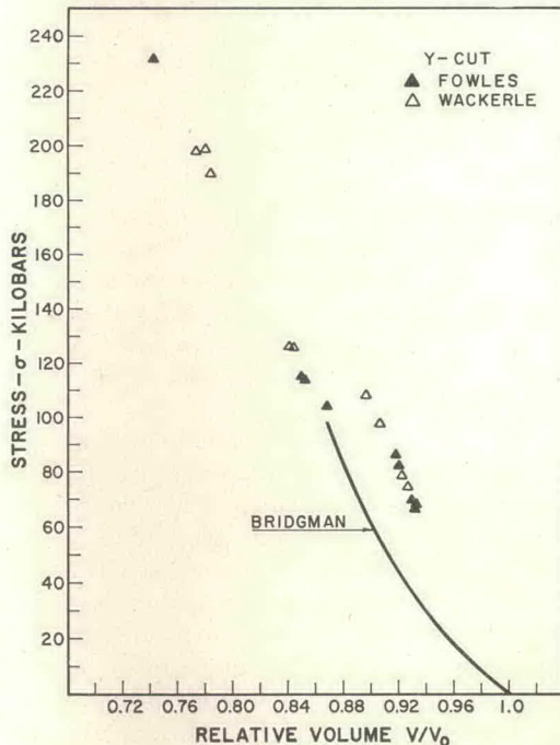
Fig. 8. Stress-volume states resulting from shock compression of Y-cut quartz. Solid curve is Bridgman's hydrostatic data.
